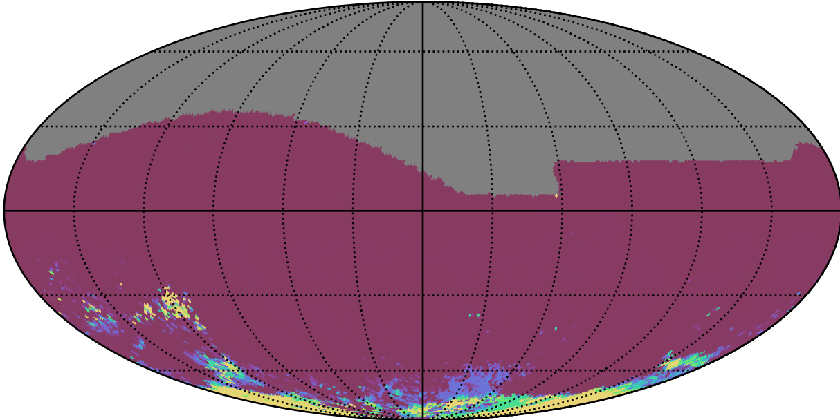
noroll_mjdp270_v3.4_10yrs All sky ri bands: 75th Percentile Intranight Timespan
