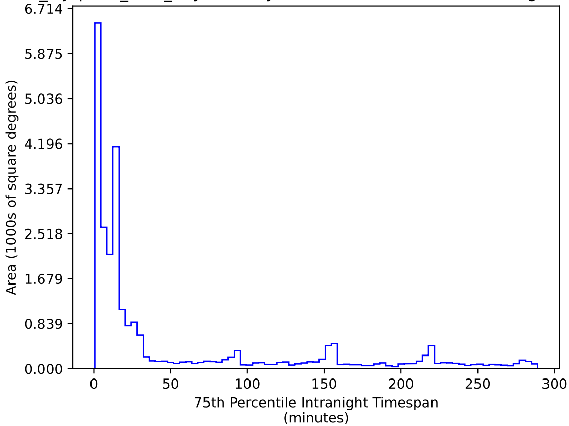
noroll_mjdp270_v3.4_10yrs All sky r band: 75th Percentile Intranight Timespan
