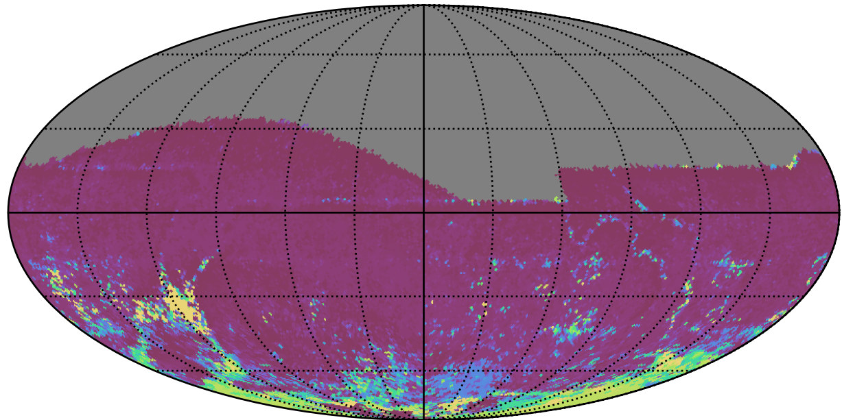
noroll_mjdp270_v3.4_10yrs All sky i band: 75th Percentile Intranight Timespan
