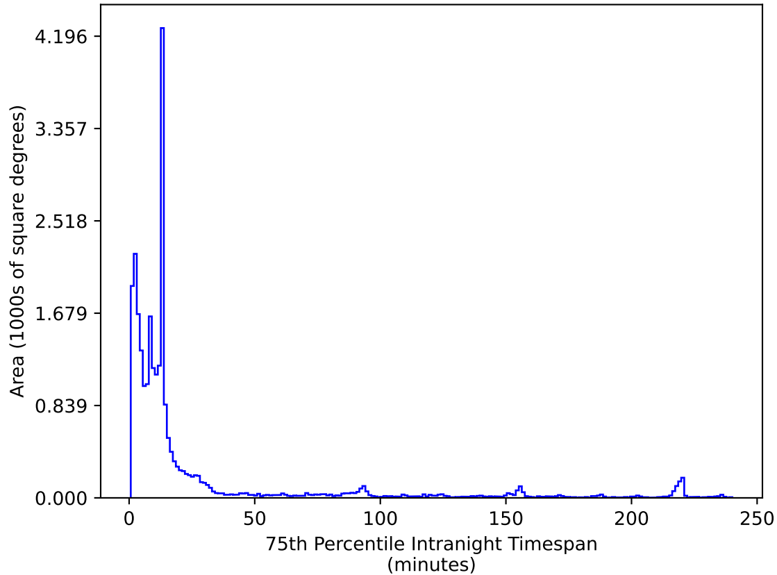
noroll_mjdp270_v3.4_10yrs All sky i band: 75th Percentile Intranight Timespan
