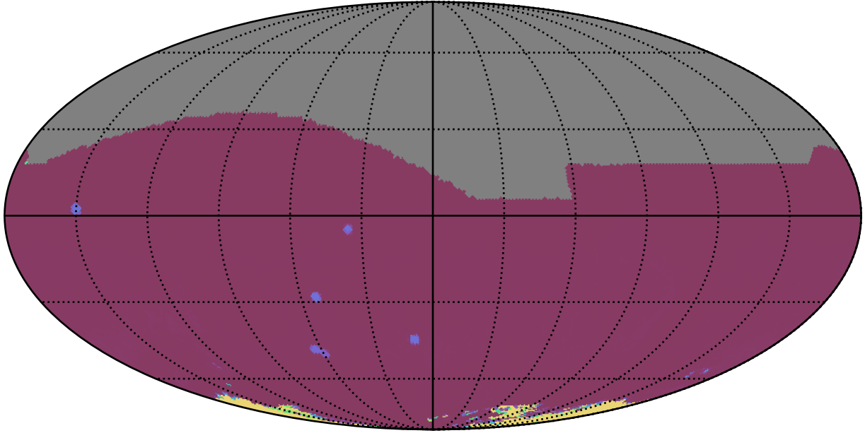
noroll_mjdp270_v3.4_10yrs All sky all bands: 75th Percentile Intranight Timespan
