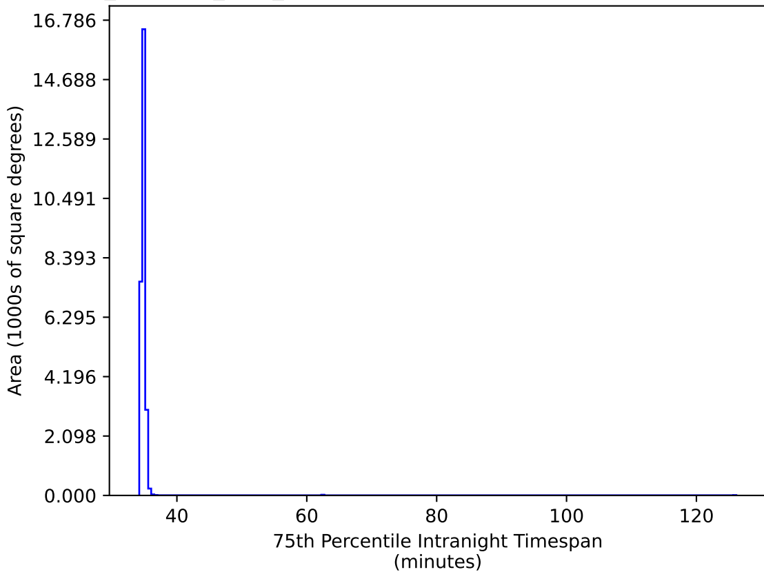
noroll_mjdp270_v3.4_10yrs All sky: 75th Percentile Intranight Timespan
