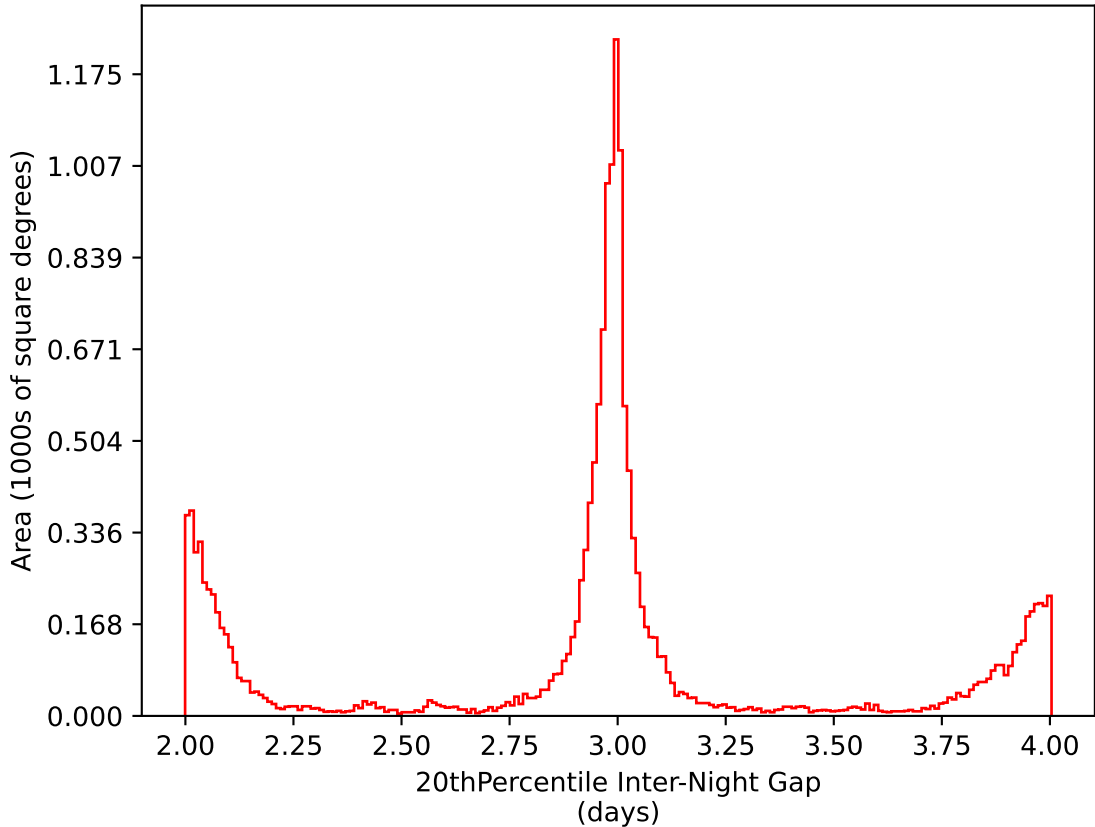
noroll_mjdp270_v3.4_10yrs WFD i band: 20thPercentile Inter-Night Gap
