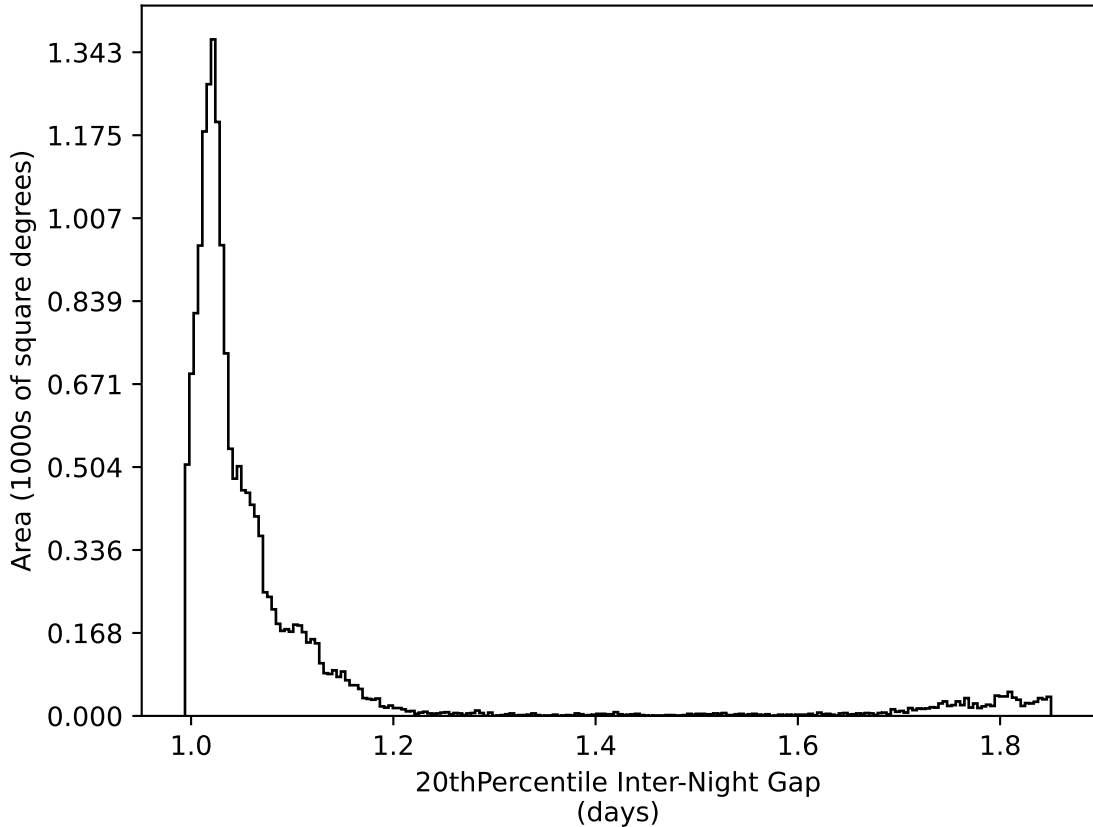
noroll_mjdp270_v3.4_10yrs WFD all bands: 20thPercentile Inter-Night Gap
