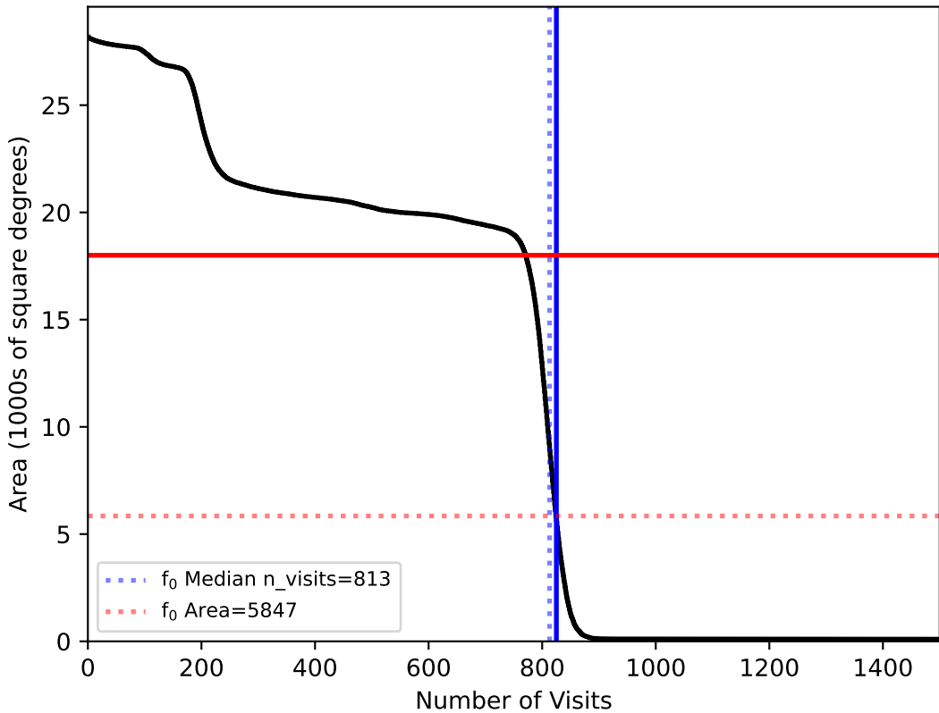
noroll_mjdp270_v3.4_10yrs : fO
