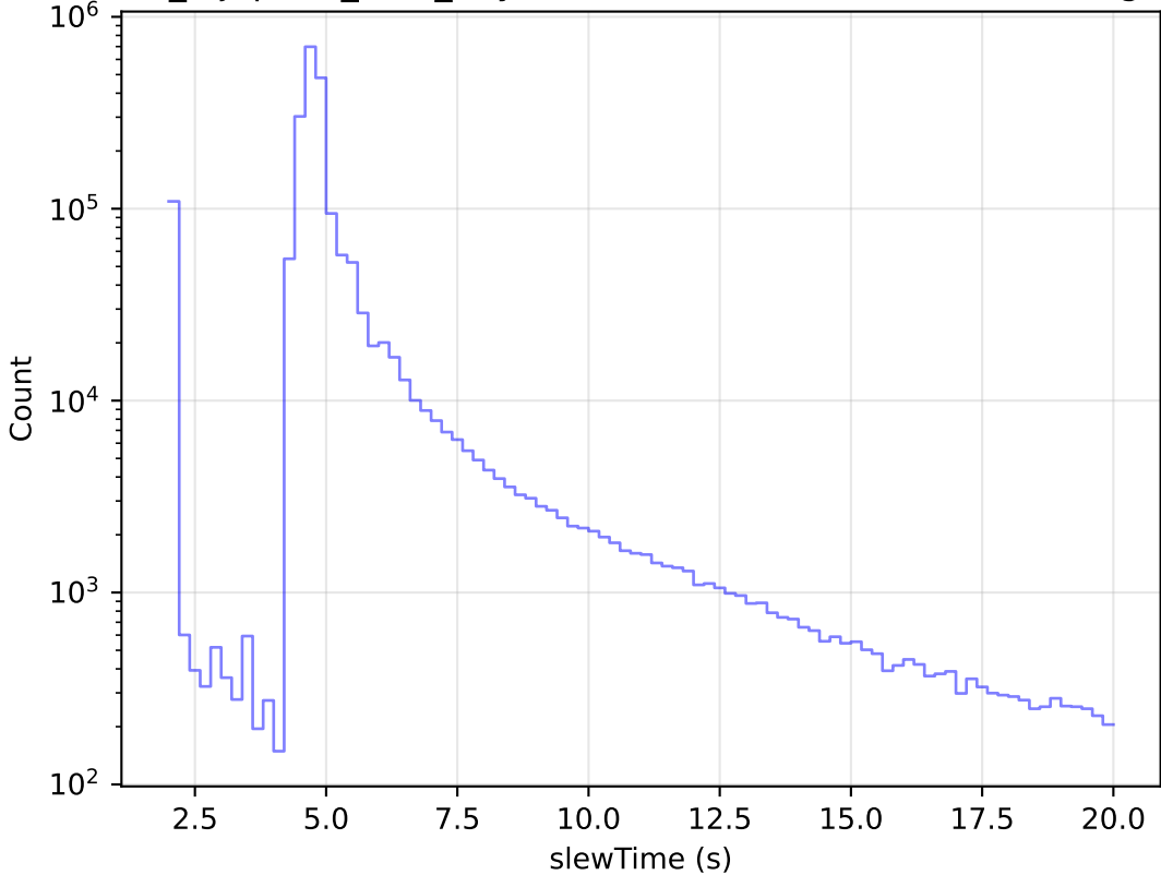
noroll_mjdp270_v3.4_10yrs All visits: Zoom Slew Time Histogram
