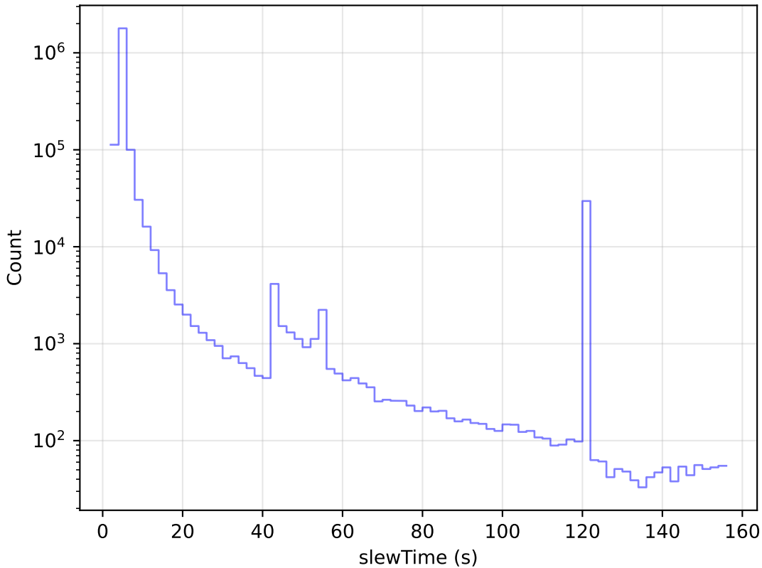
noroll_mjdp270_v3.4_10yrs All visits: Slew Time Histogram
