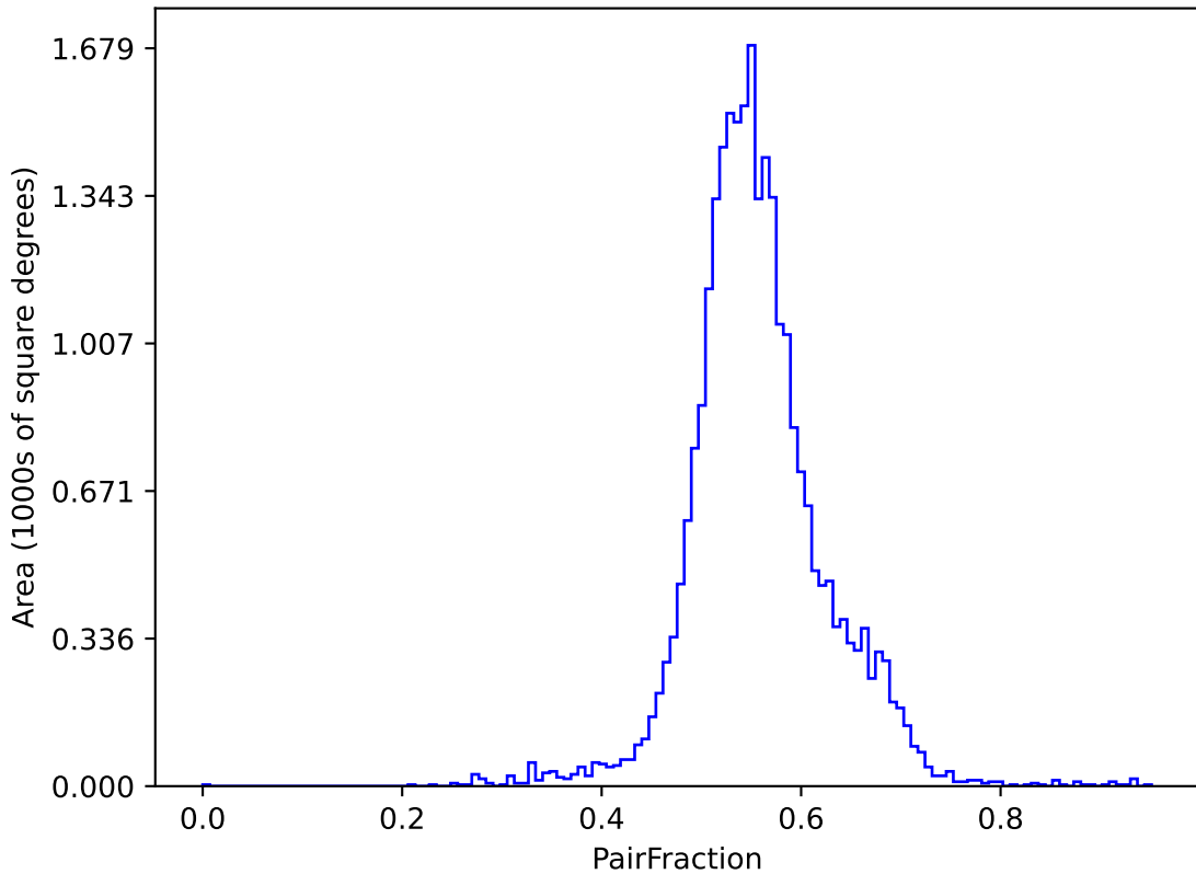
noroll_mjdp270_v3.4_10yrs (g or r or i): PairFraction
