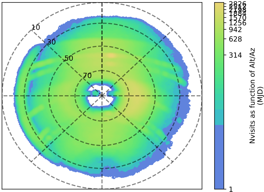
noroll_mjdp270_v3.4_10yrs r: Nvisits as function of Alt/Az
