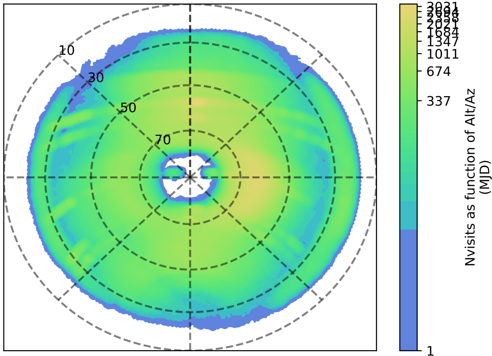
noroll_mjdp270_v3.4_10yrs i: Nvisits as function of Alt/Az
