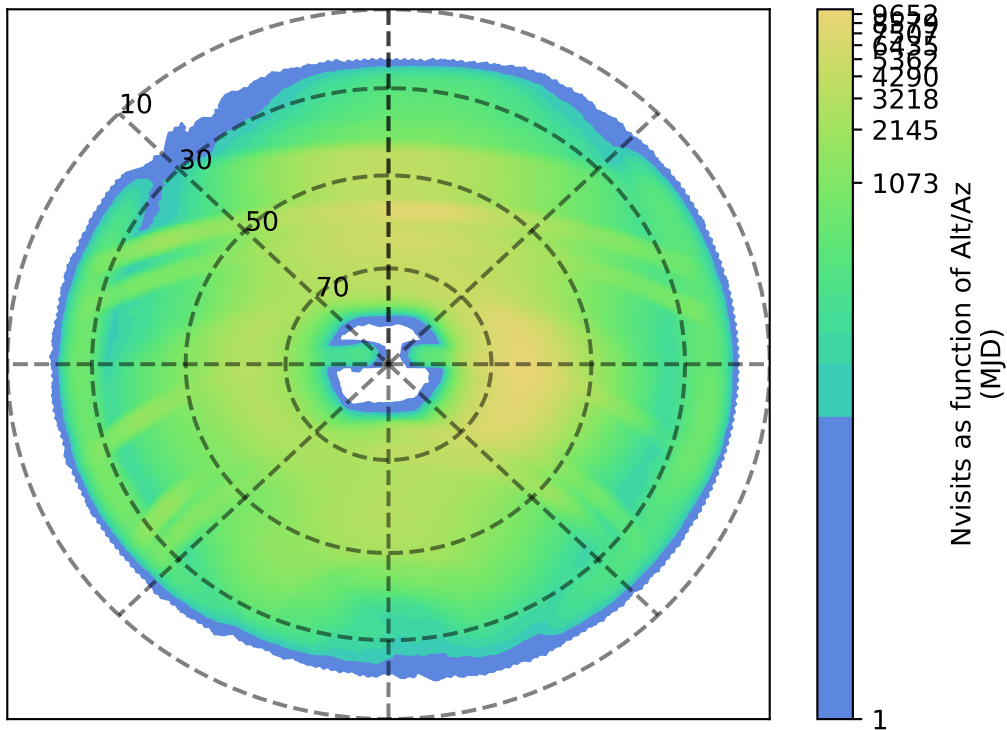
noroll_mjdp270_v3.4_10yrs : Nvisits as function of Alt/Az
