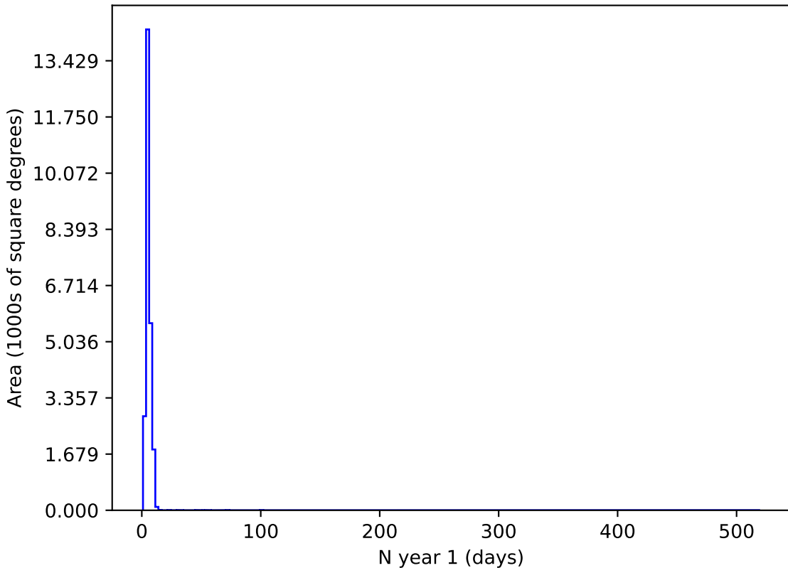
noroll_mjdp270_v3.4_10yrs u and night < 365: N year 1
