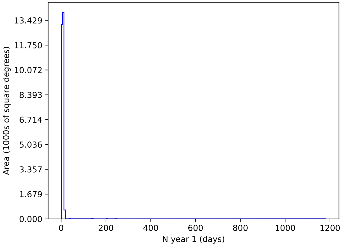
noroll_mjdp270_v3.4_10yrs g and night < 365: N year 1
