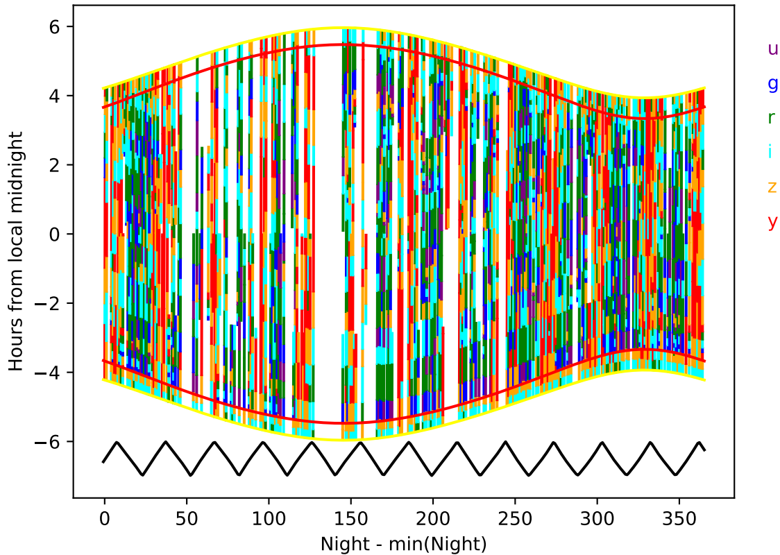
noroll_mjdp270_v3.4_10yrs year 8-9: Hourglass
