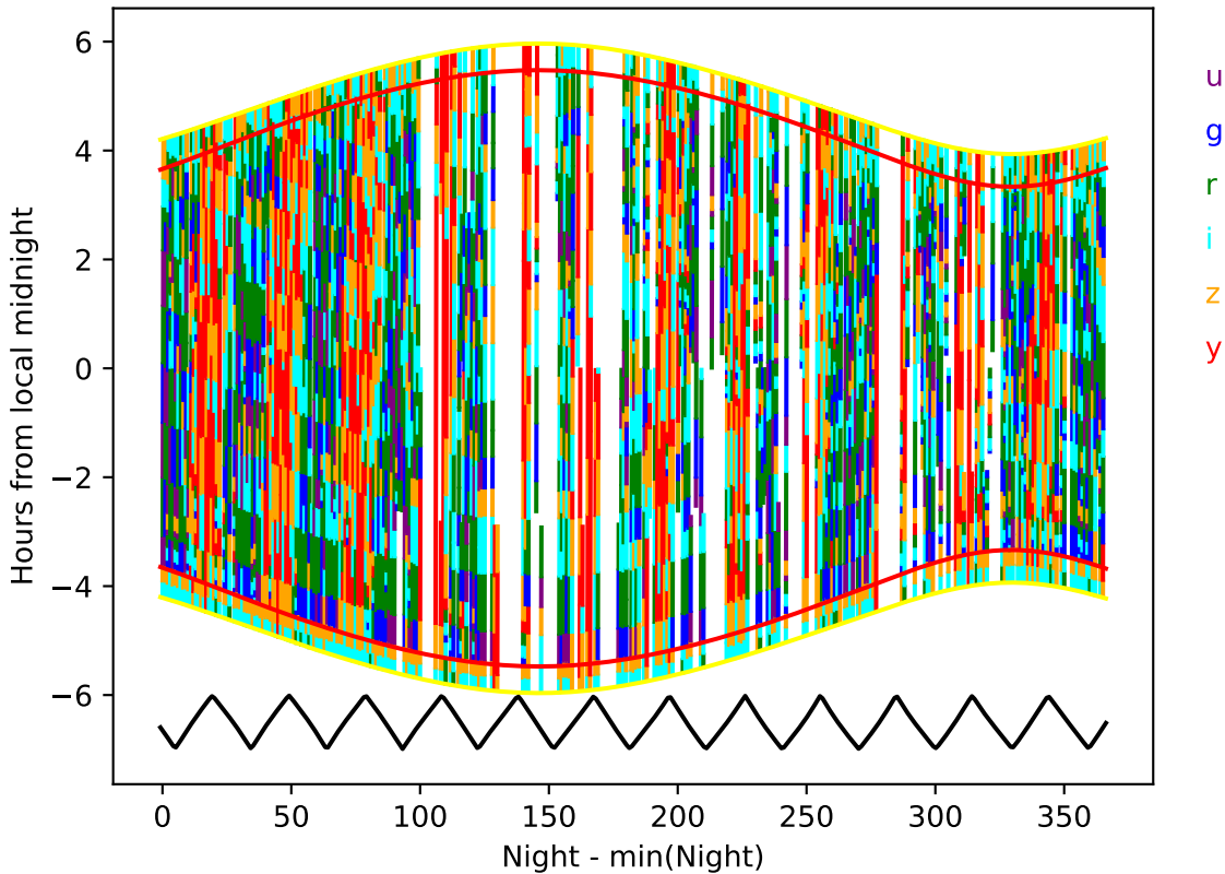
noroll_mjdp270_v3.4_10yrs year 7-8: Hourglass
