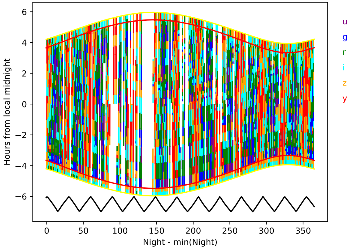
noroll_mjdp270_v3.4_10yrs year 6-7: Hourglass
