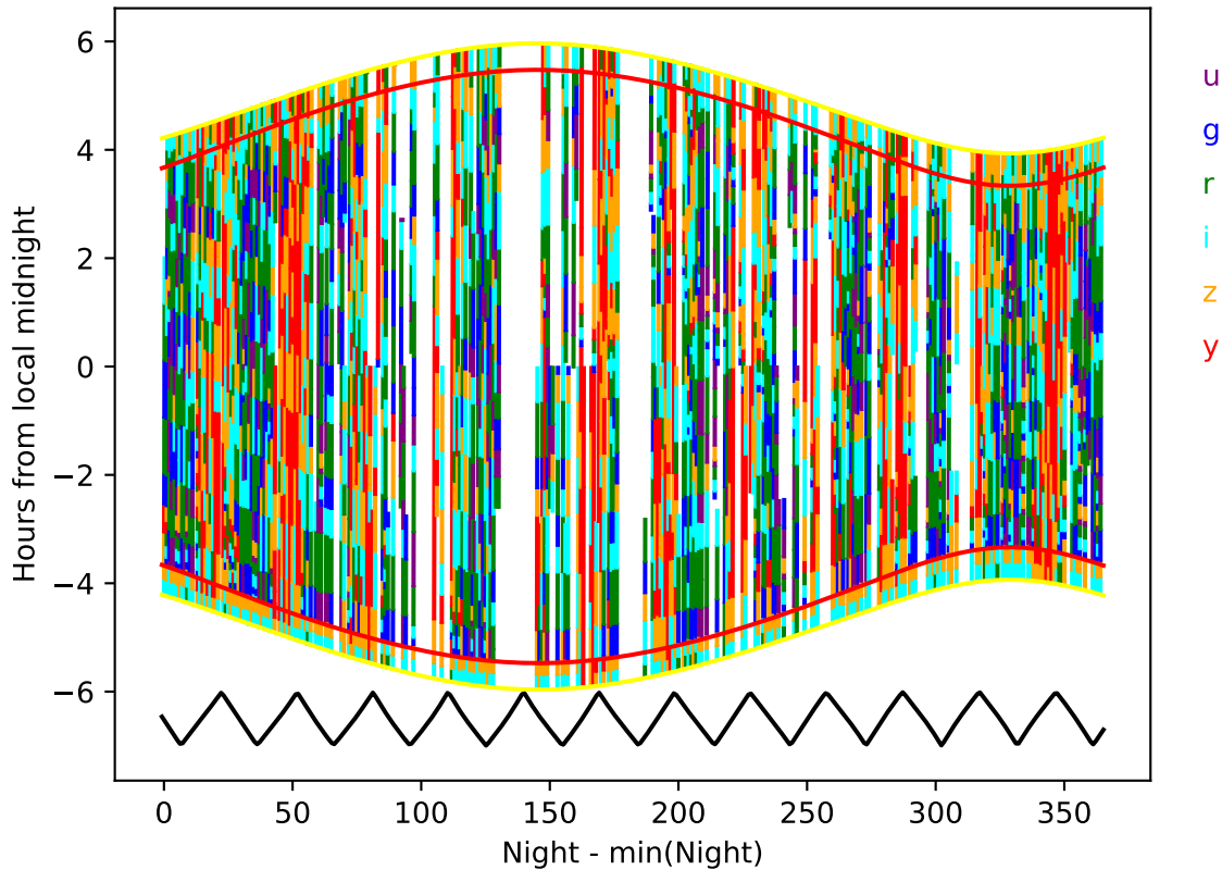
noroll_mjdp270_v3.4_10yrs year 4-5: Hourglass
