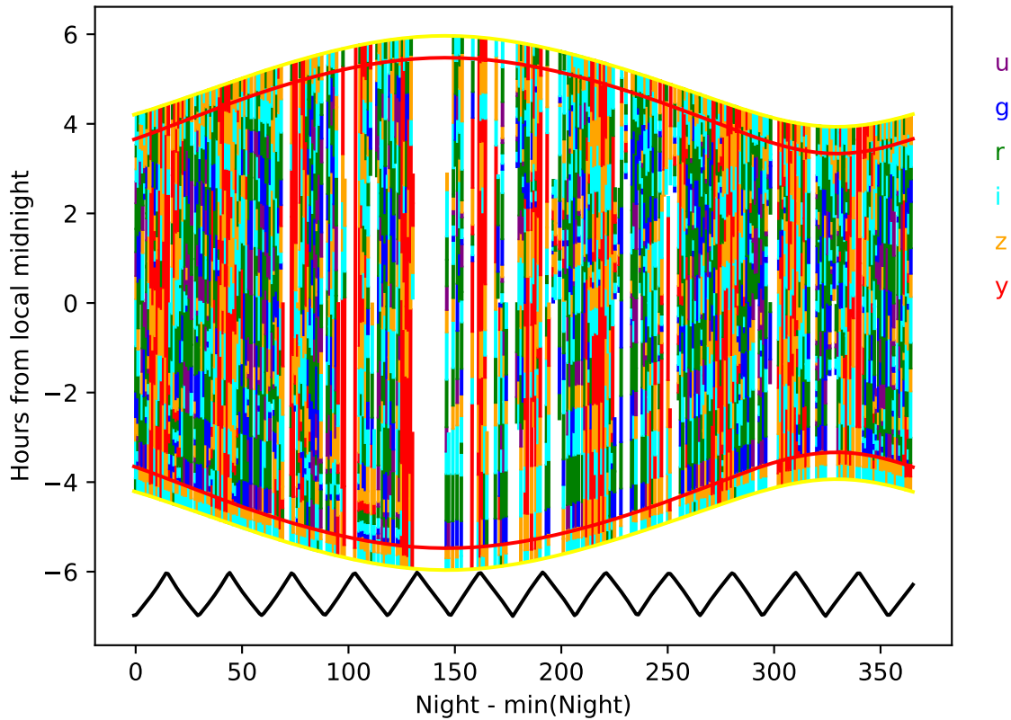
noroll_mjdp270_v3.4_10yrs year 2-3: Hourglass
