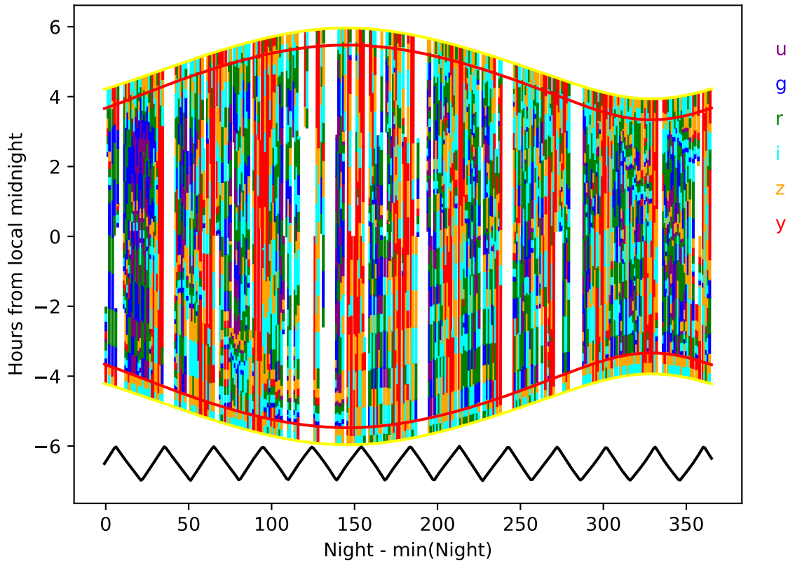
noroll_mjdp270_v3.4_10yrs year 0-1: Hourglass
