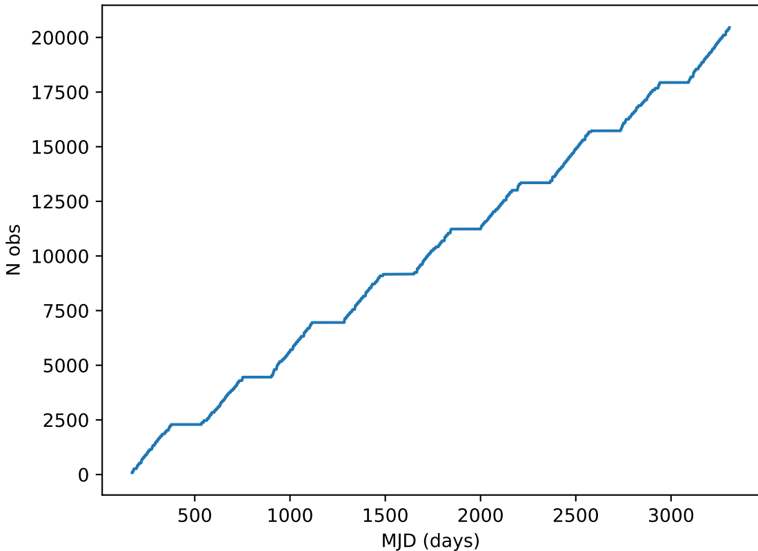
noroll_mjdp270_v3.4_10yrs note like DD:XMM_LSS%: Cumulative
