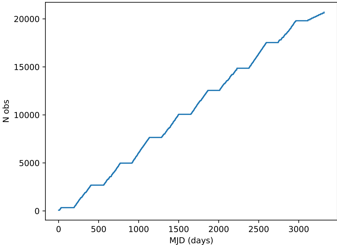
noroll_mjdp270_v3.4_10yrs note like DD:ECDFS%: Cumulative
