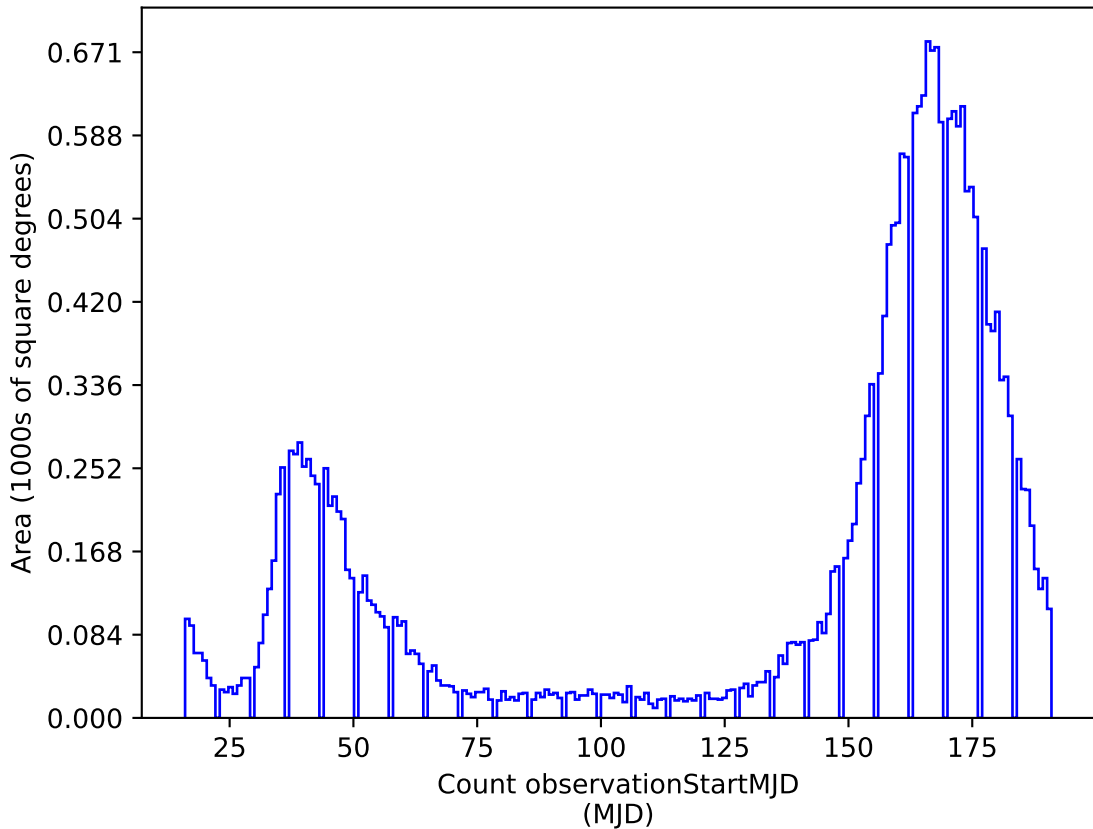
noroll_mjdp270_v3.4_10yrs z: Count observationStartMJD
