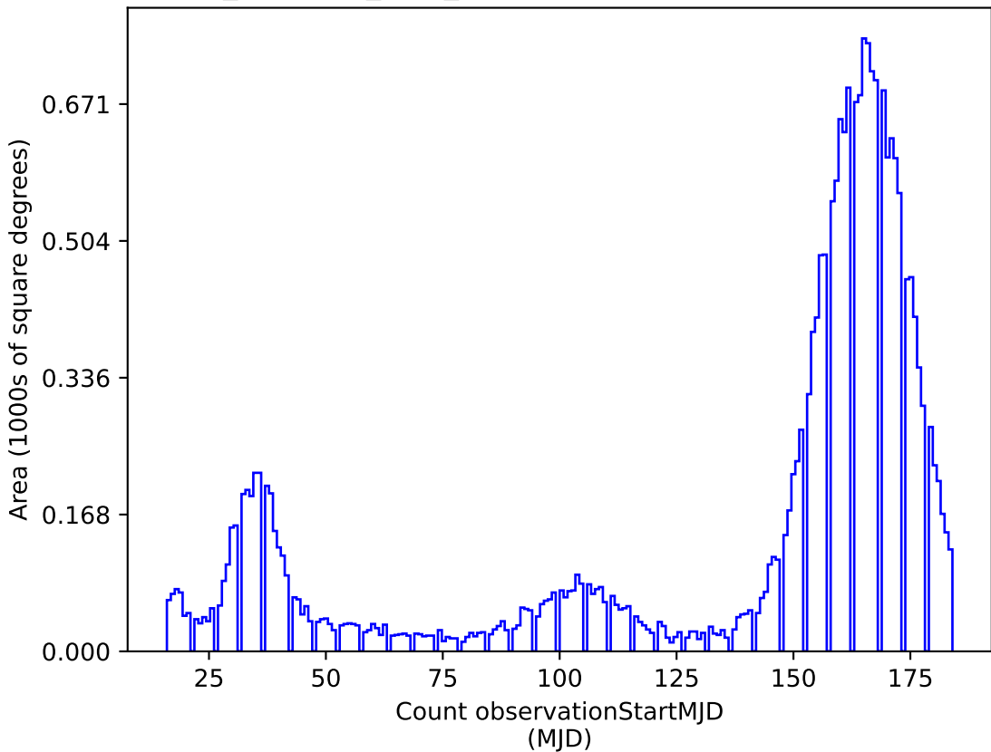
noroll_mjdp270_v3.4_10yrs y: Count observationStartMJD
