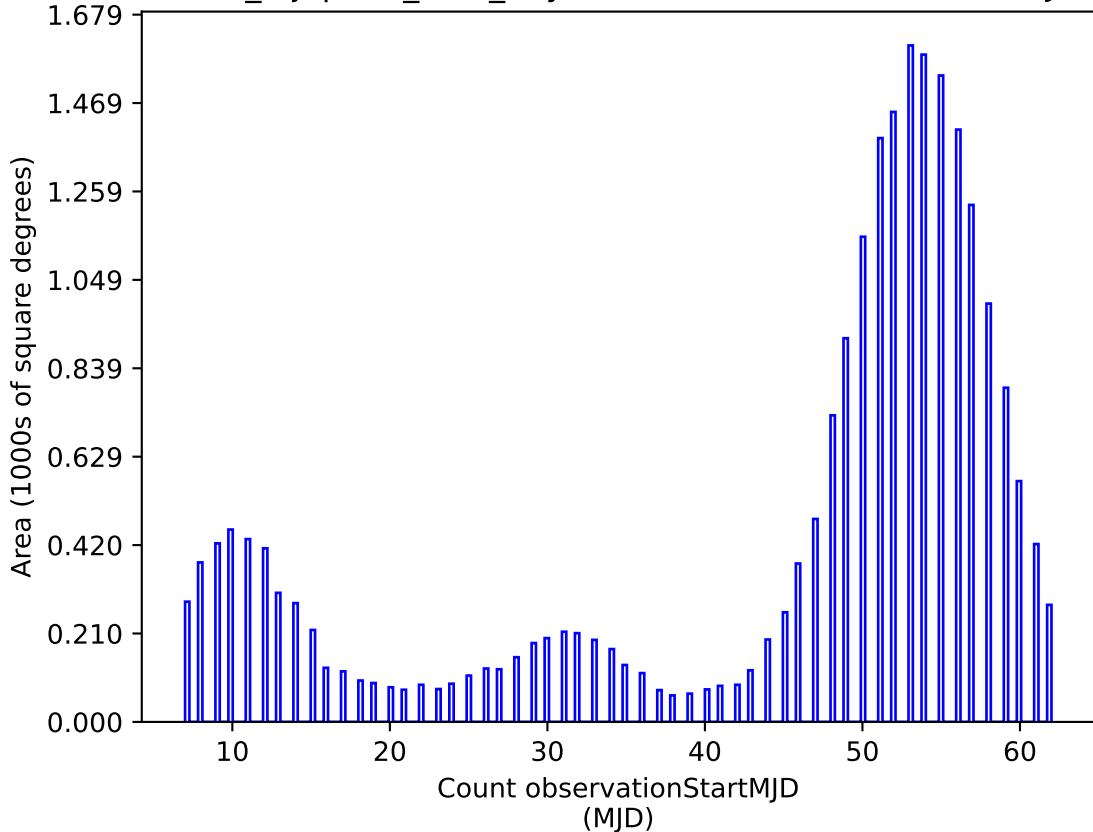
noroll_mjdp270_v3.4_10yrs u: Count observationStartMJD
