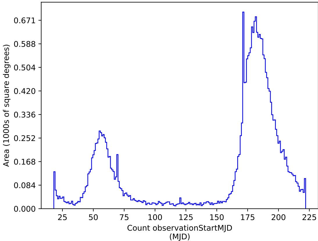
noroll_mjdp270_v3.4_10yrs r: Count observationStartMJD
