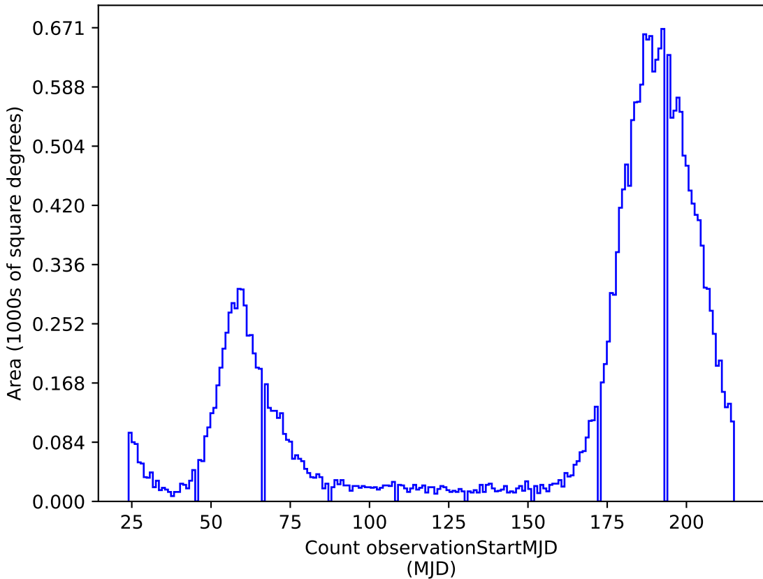
noroll_mjdp270_v3.4_10yrs i: Count observationStartMJD
