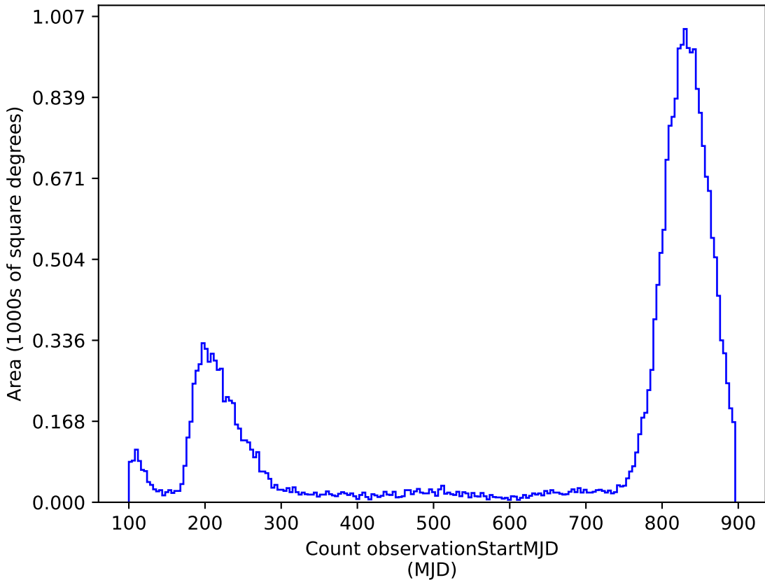
noroll_mjdp270_v3.4_10yrs : Count observationStartMJD
