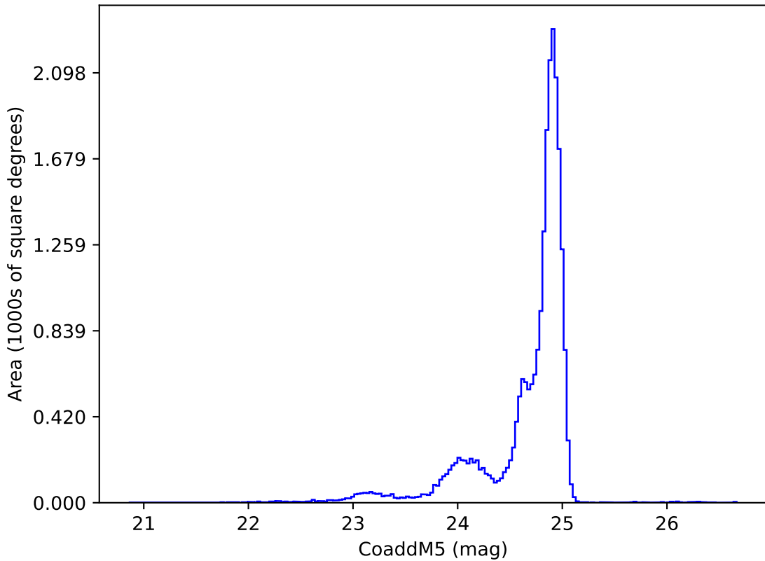
noroll_mjdp270_v3.4_10yrs y: CoaddM5
