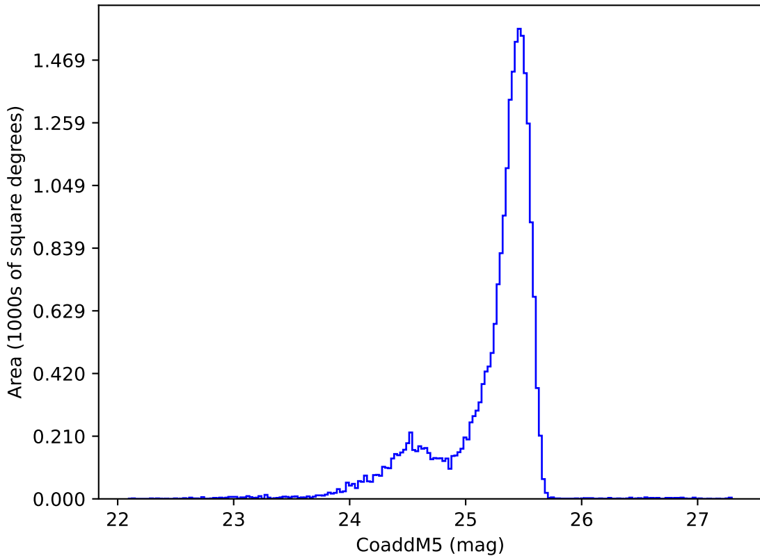
noroll_mjdp270_v3.4_10yrs u: CoaddM5
