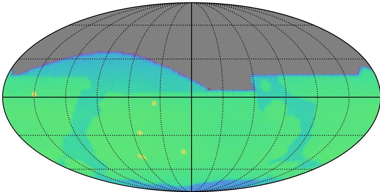
noroll_mjdp270_v3.4_10yrs r: CoaddM5
