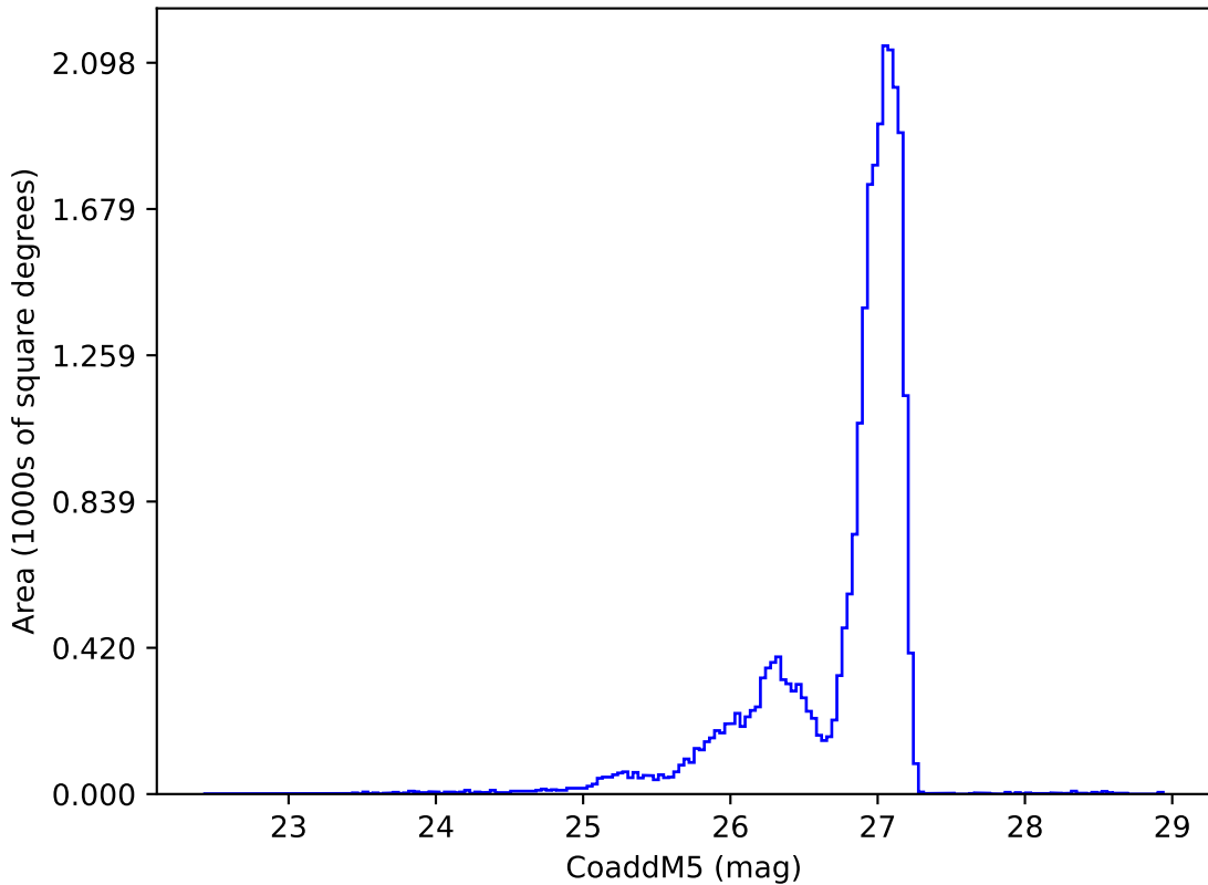
noroll_mjdp270_v3.4_10yrs r: CoaddM5
