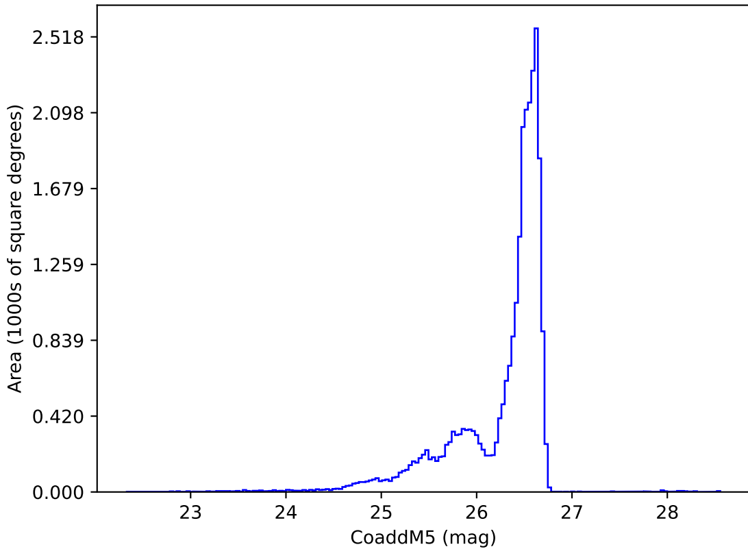
noroll_mjdp270_v3.4_10yrs i: CoaddM5
