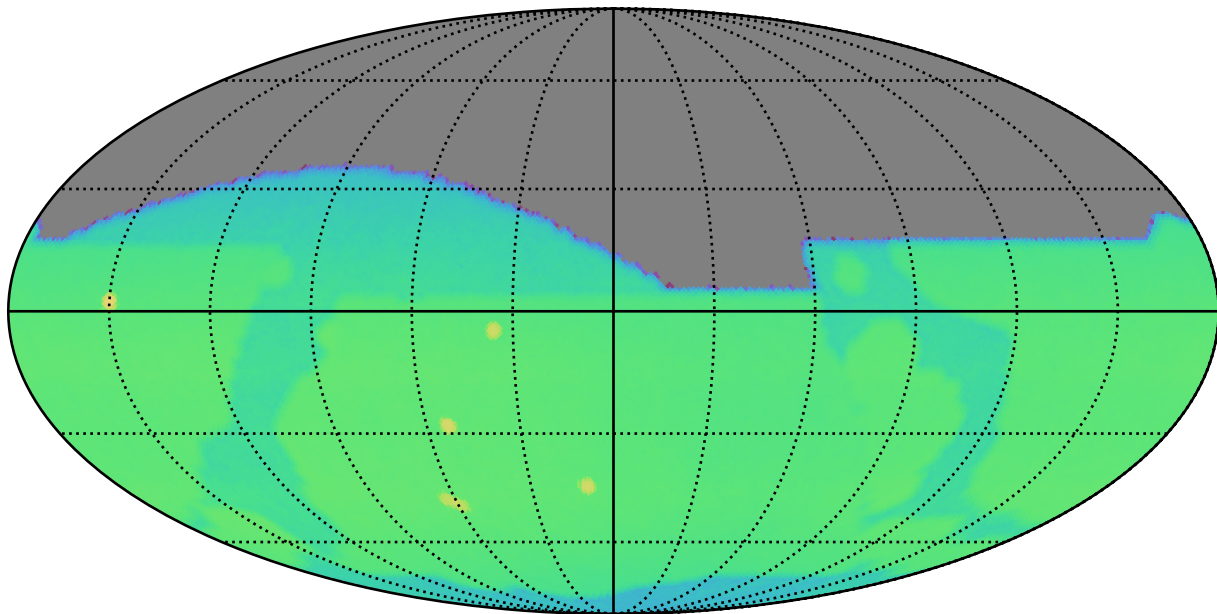
noroll_mjdp270_v3.4_10yrs : CoaddM5
