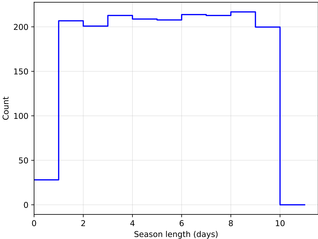
noroll_mjdp270_v3.4_10yrs DD:ECDFS all bands: SeasonLength
