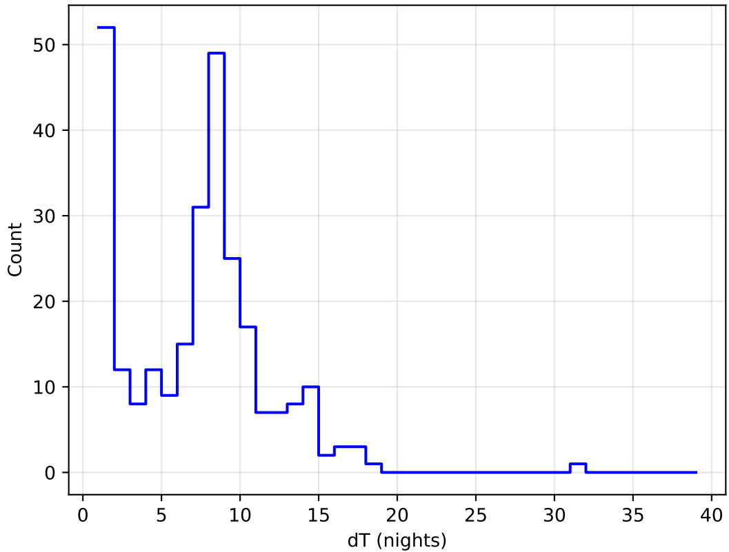
noroll_mjdp270_v3.4_10yrs all bands: DD:XMM_LSS Delta Nights Histogram
