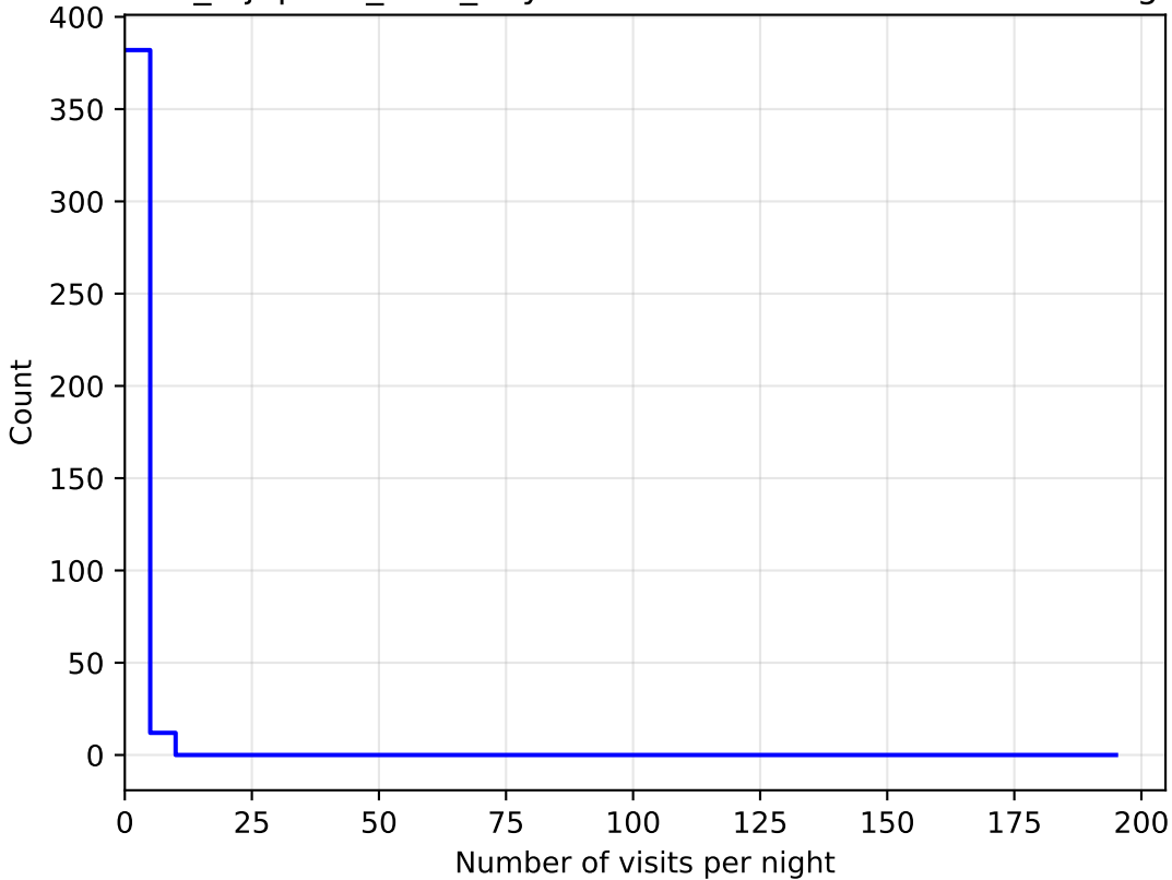
noroll_mjdp270_v3.4_10yrs all bands: DD:WFD NVisitsPerNight
