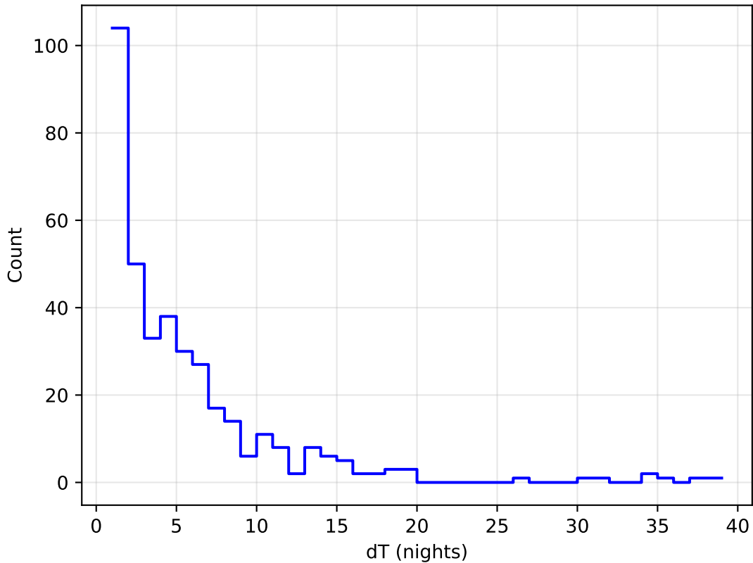
noroll_mjdp270_v3.4_10yrs all bands: DD:WFD Delta Nights Histogram
