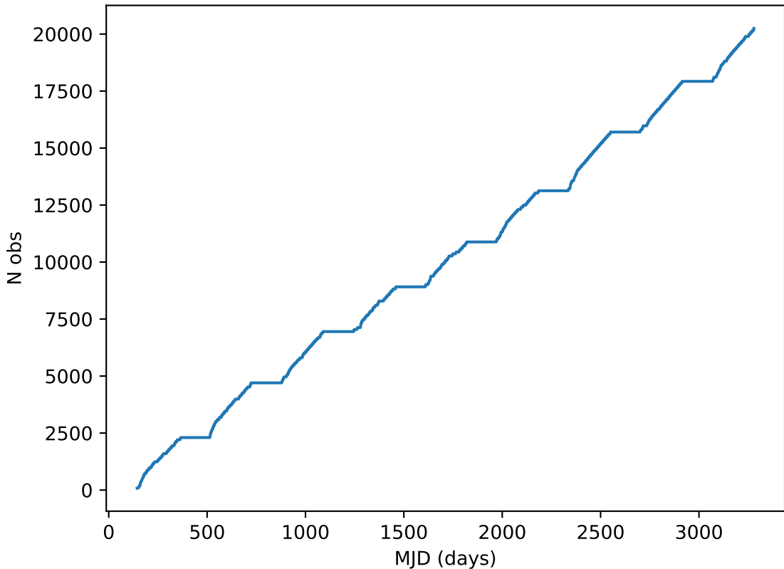
noroll_mjdp270_v3.4_10yrs all bands: DD:ELAISS1 Cumulative NVisits
