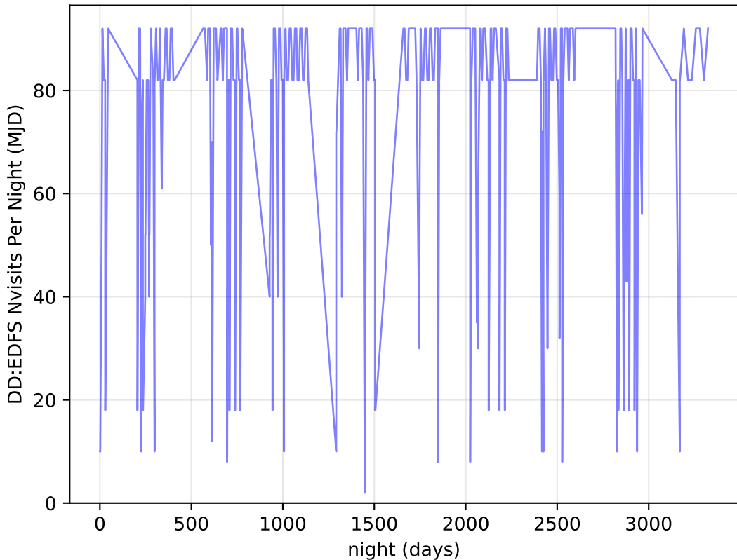
noroll_mjdp270_v3.4_10yrs all bands: DD:EDFS Nvisits Per Night
