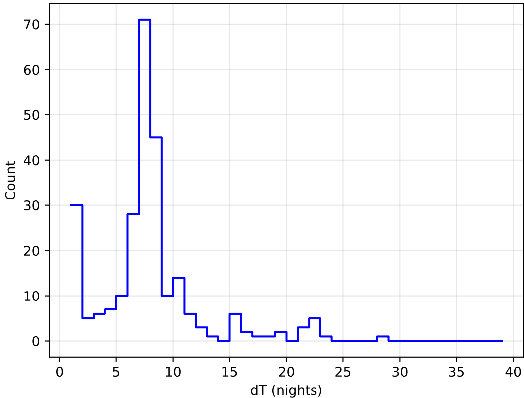
noroll_mjdp270_v3.4_10yrs all bands: DD:EDFS Delta Nights Histogram
