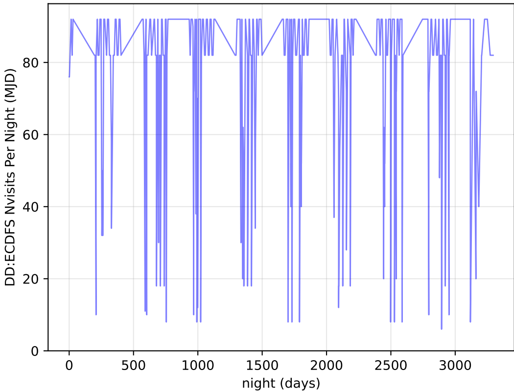
noroll_mjdp270_v3.4_10yrs all bands: DD:ECDFS Nvisits Per Night
