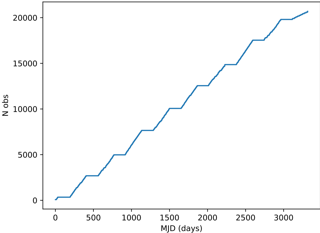
noroll_mjdp270_v3.4_10yrs all bands: DD:ECDFS Cumulative NVisits
