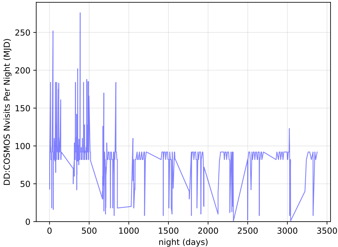
noroll_mjdp270_v3.4_10yrs all bands: DD:COSMOS Nvisits Per Night
