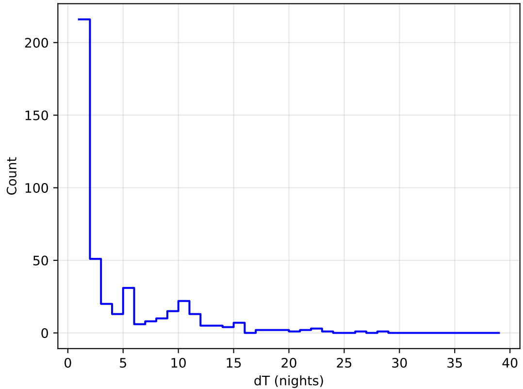
noroll_mjdp270_v3.4_10yrs all bands: DD: COSMOS Delta Nights Histogram
