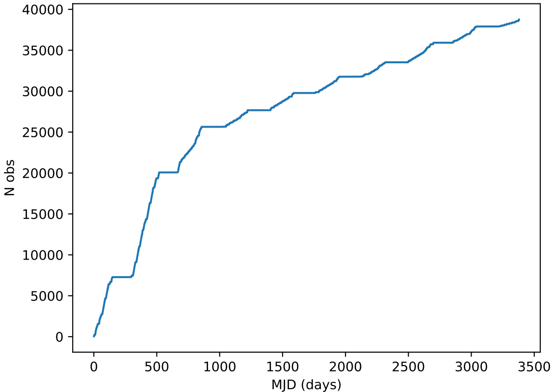
noroll_mjdp270_v3.4_10yrs all bands: DD: COSMOS Cumulative NVisits
