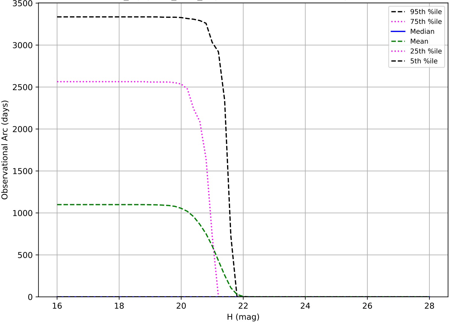
noroll_mjdp180_v3.4_10yrs: Observational Arc Length Vatira
